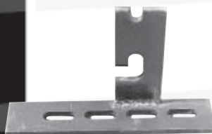
Quick Attach Foot (for Gating)
